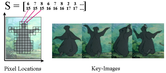
Figure 5: Left side illustrates how the shape vector S is used to index all pixel locations of the cartoon. Right side shows four key-shape examples. ©Disney.
